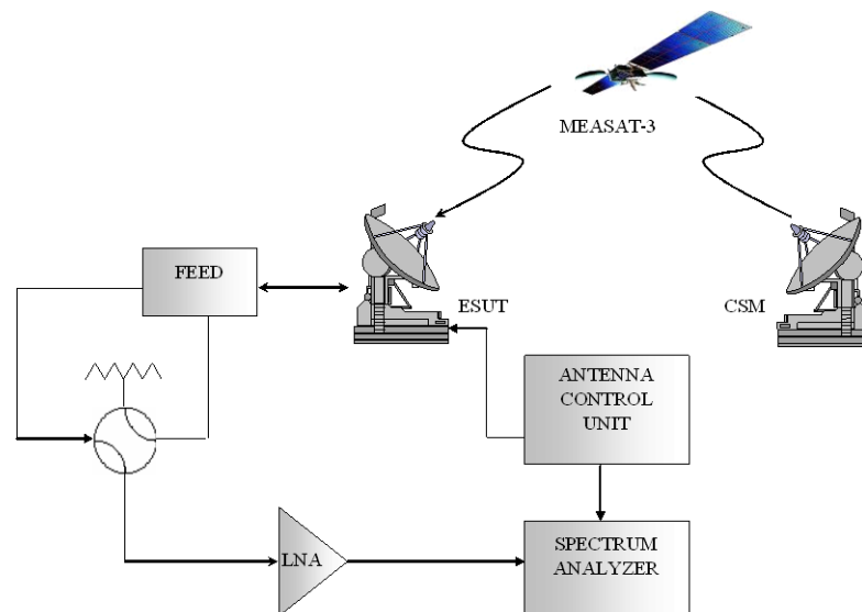
Figure 3: Receive Antenna Side lobe Pattern Measurement Setup
